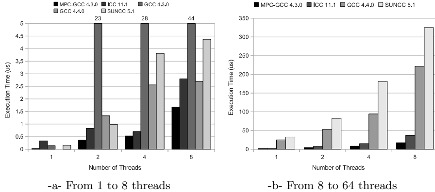
Fig. 3. Overhead of OpenMP Parallel Construct on 8-core Nehalem Architecture
