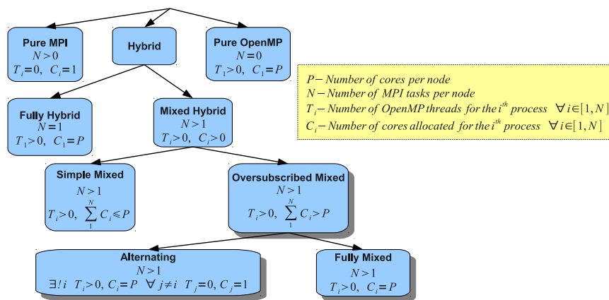
Fig. 1. Extended Taxonomy of Hybrid MPI/OpenMP Programming Models
